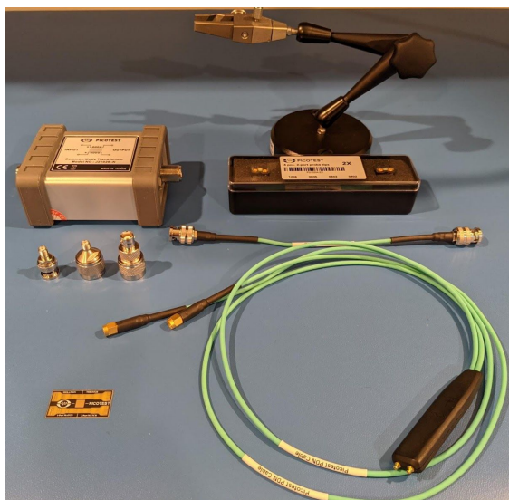
Fig. 2 - Picotest PDN cables, J2102B ground isolator, calibration substrate, P2102A probe, P2102A probe tips, and probe holder for measurement.
